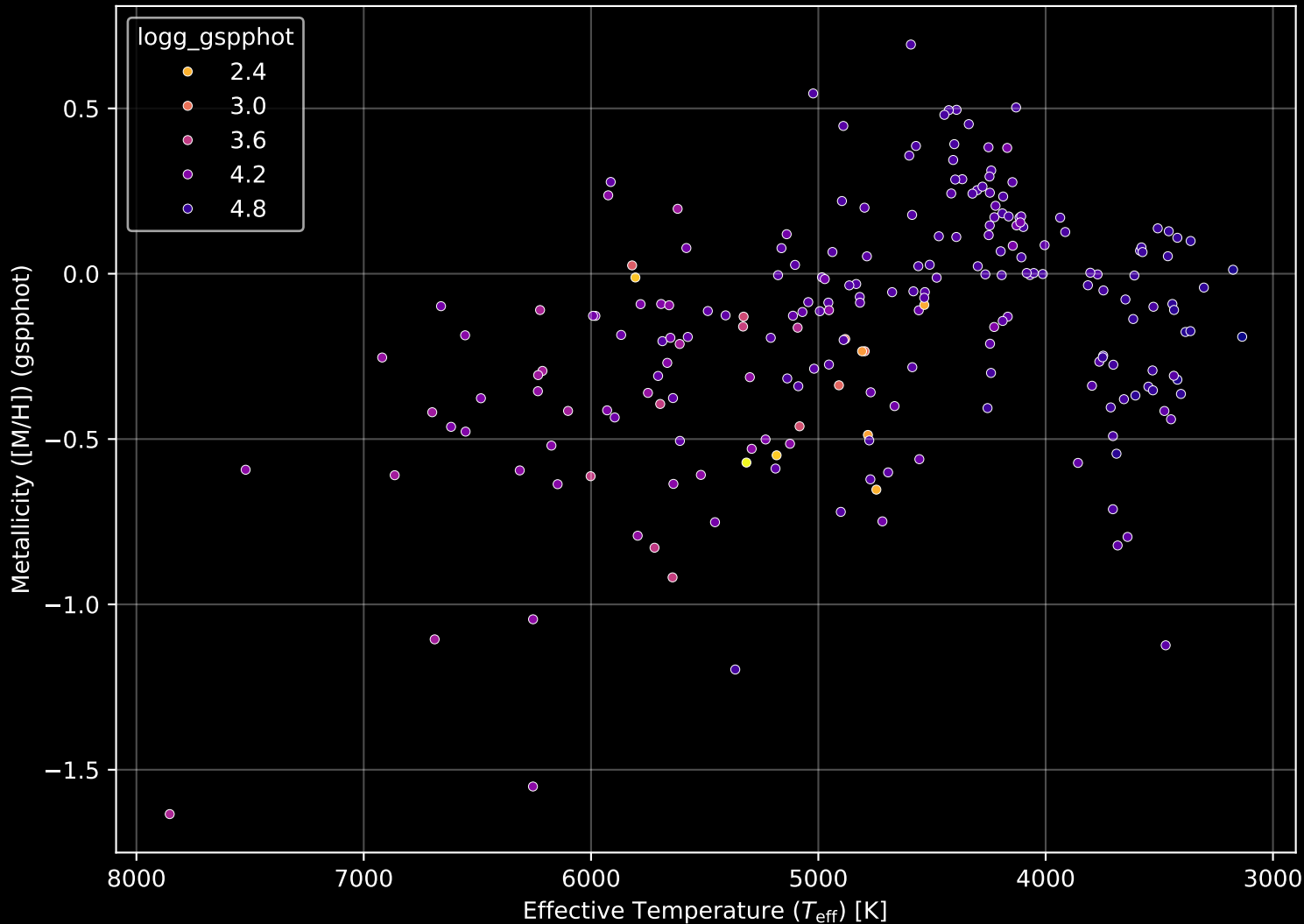
APOGEE DR17 Field: [K2_C1_258+53_btx] Stellar Population Parameters (n= 220)
