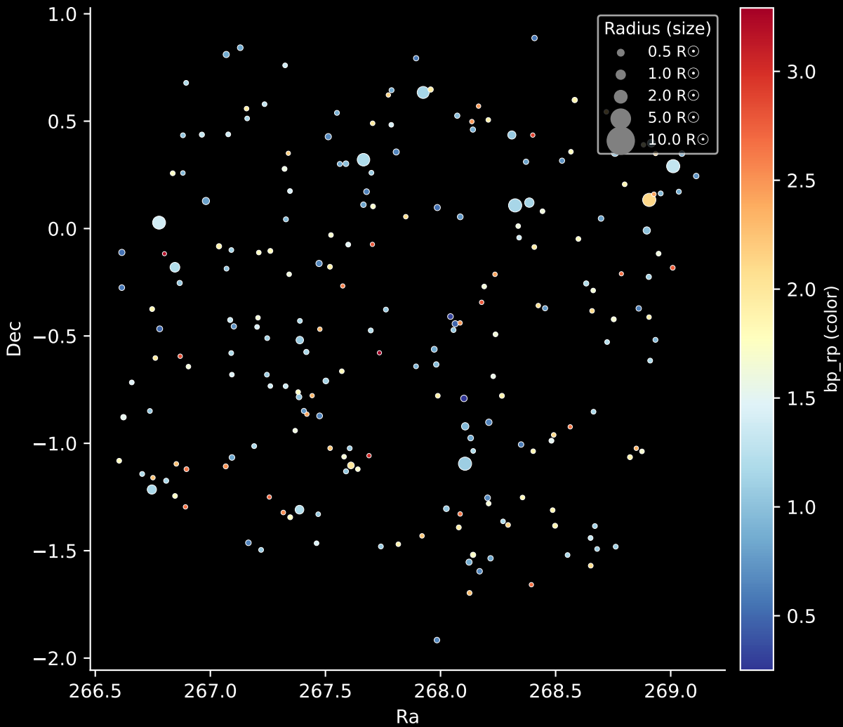
APOGEE DR17 Field: [K2_C1_258+53_btx] Stars: 220
