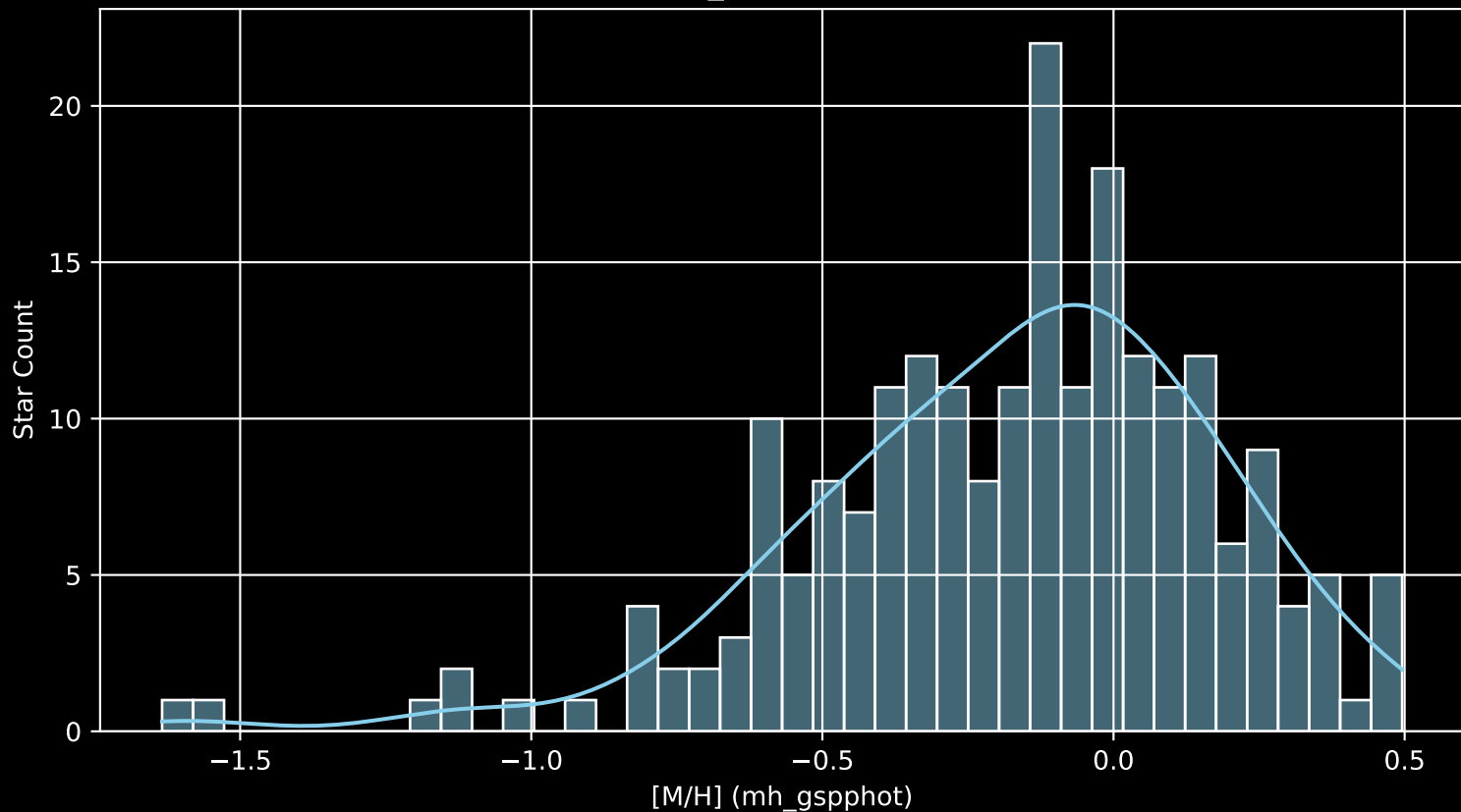
APOGEE DR17 Field: [K2_C1_258+53_btx [M/H] (mh_gspphot) (n= 217)
