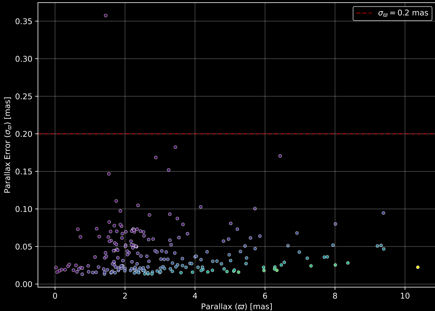
APOGEE DR17 Field: [K2_C1_258+53_btx] Parallax Quality (n= 220)
