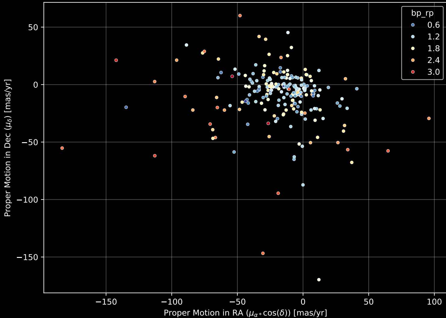
APOGEE DR17 Field: [K2_C1_258+53_btx] Proper Motion Diagram (n= 220)
