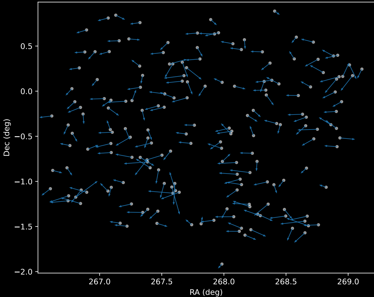
APOGEE DR17 Cluster 0 Proper Motion Vectors (n=182)
