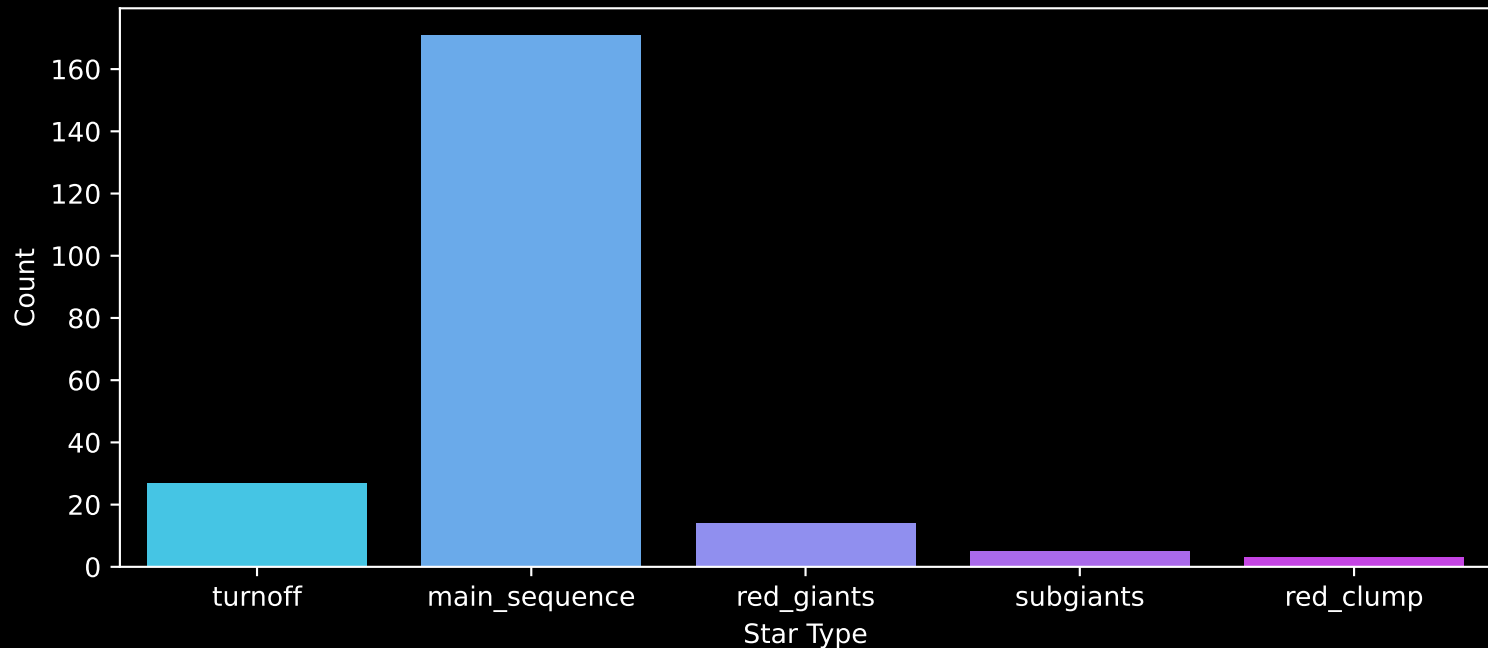
APOGEE DR17 Field: [K2_C1_258+53_btx] Count plot of Star Type
