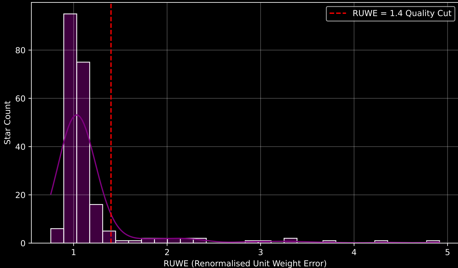
GAPOGEE DR17 Field [K2_C1_258+53_btx] RUWE Distribution (n= 216)
